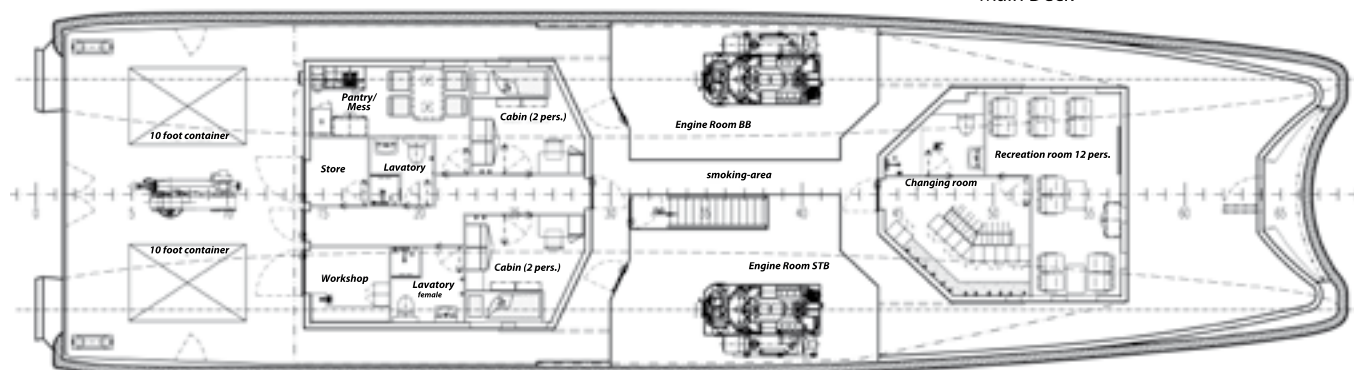
Main Deck
