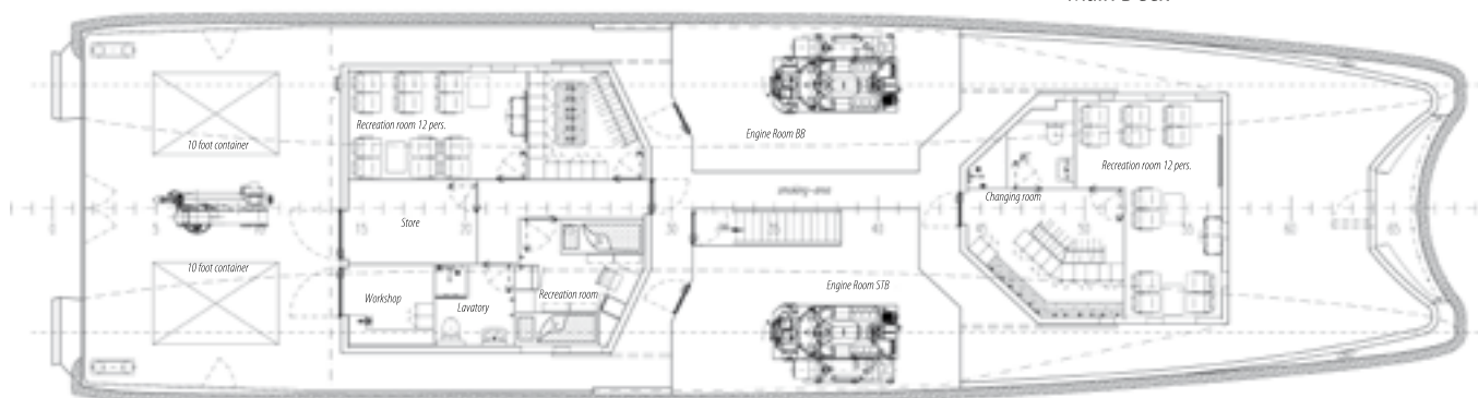
Main Deck
